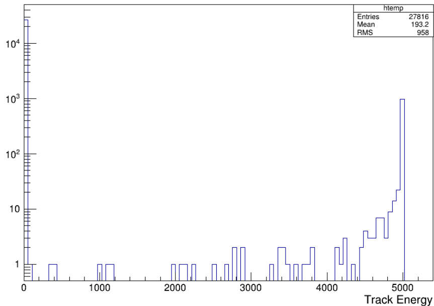
Electron Track Energy on Si-Detector
