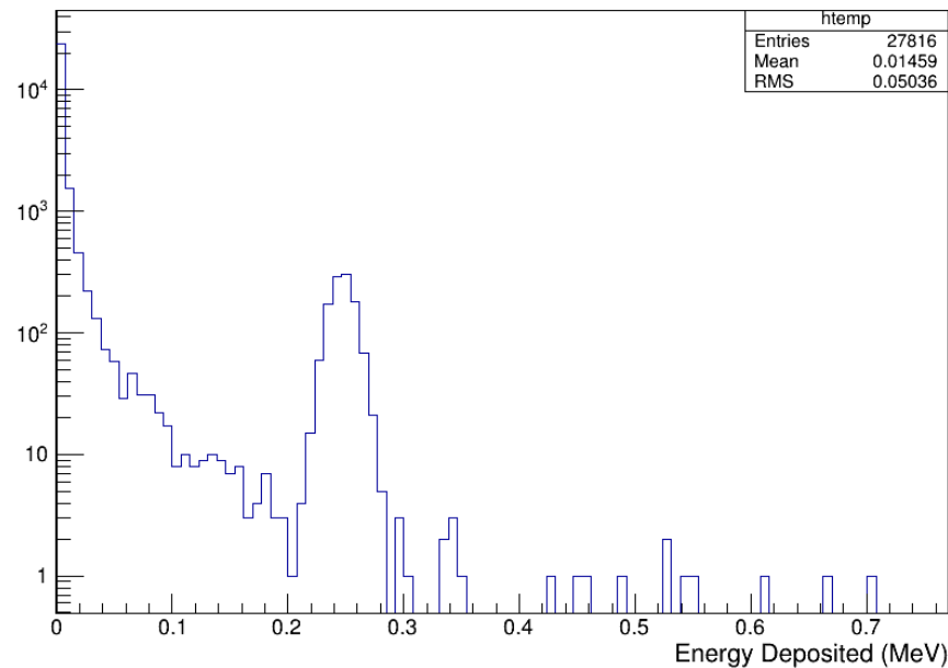
Total Energy Deposited in Si-Detector: electron
